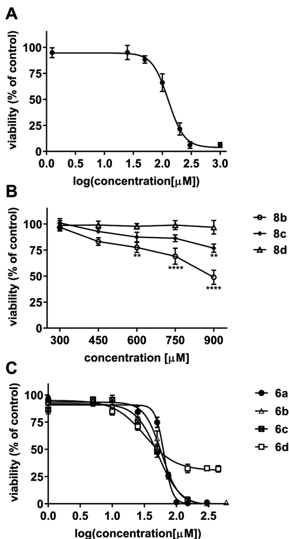
Fig. 2. Dose-response curves showing the effects of synthetic BCFAs on the viability of MCF-7 breast cancer cells after 48 h treatment. A) 13-MTD, B) saturated BCFAs 8b-d, C) unsaturated BCFAs 6a-d. Data represents the mean \pm SEM of at least 3 independent experiments. ** P < 0.01 , **** P < 0.0001 , comparison of the indicated compound to the vehicle control.
