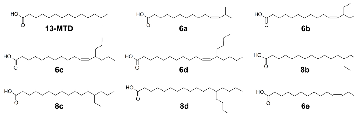
Fig. 1. Chemical structures of branched chain fatty acids used in this study.
