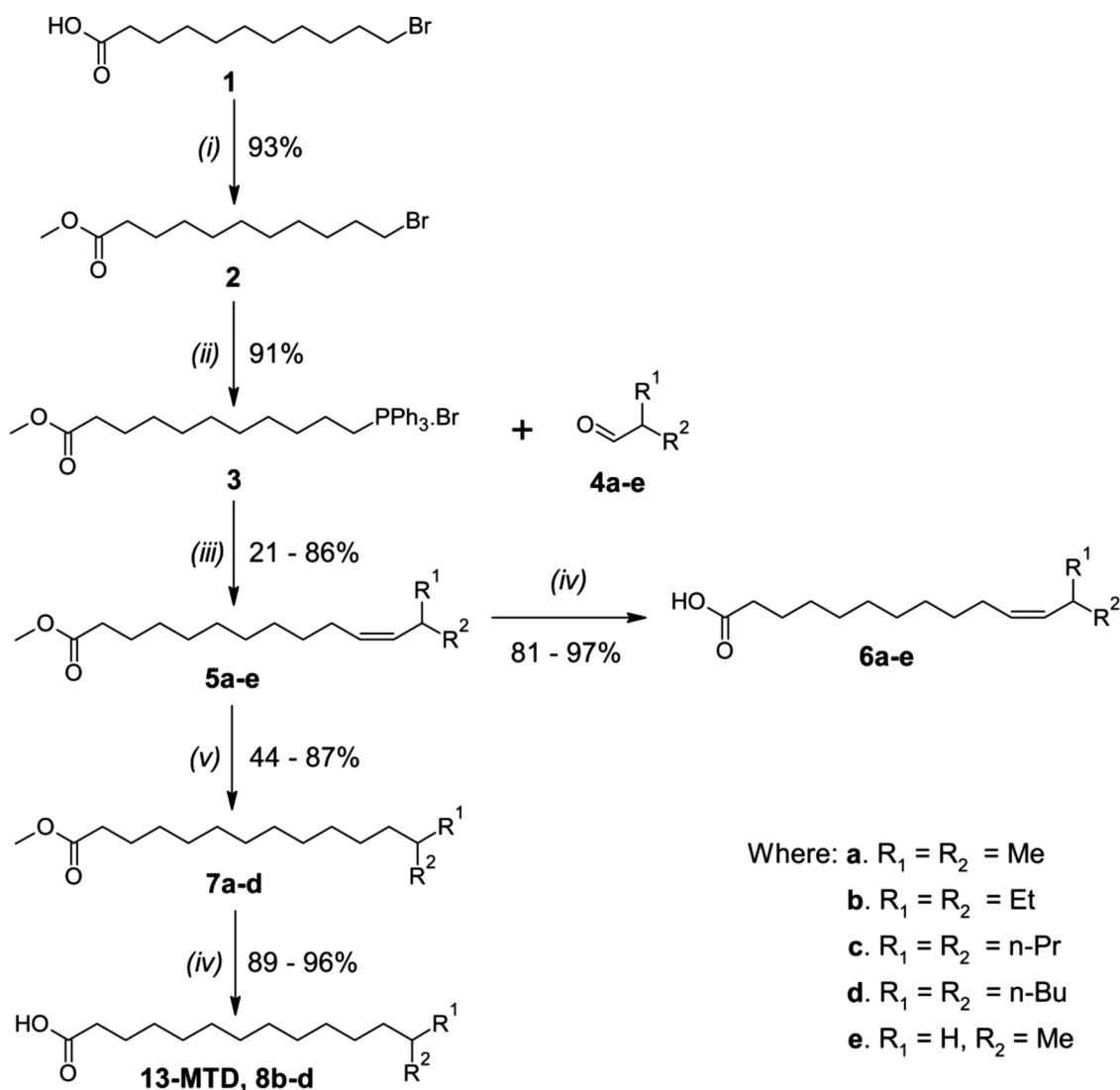
Scheme 1. Synthesis of the fatty acids 13-MTD 8b-d and 6a-e. Reagents and conditions (i) AcCl, methanol, rt, 4 h; (ii) \text{PPh}_3 , 140 °C, 20 h; (iii) \text{NaN}(\text{TMS})_2 , THF, -78 °C to rt, 2 h; (iv) 1.5 M NaOH, ethanol, 40 °C, 4 h; (v) Pd/C, hydrogen, rt, 20 h.
