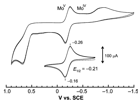
Figure 4. Cyclic voltammograms of (\text{NEt}_4)_2[\text{Mo}^{\text{IV}}\text{O}(1,2\text{-S}_2\text{-3-CH}_3\text{CONHC}_6\text{H}_3)_2] ( 5a ) in DMF. Two scans were obtained in the different ranges of the potential.
