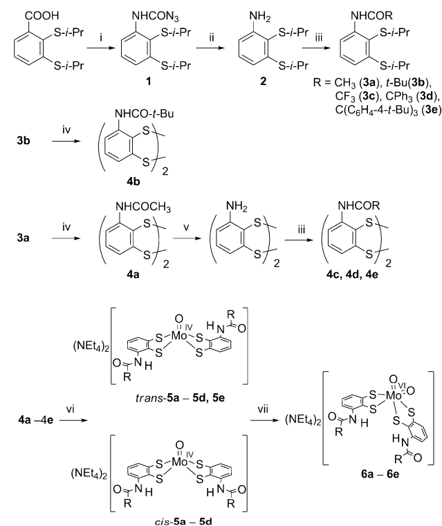
Scheme 1. Synthetic Route of the Disulfides and the Molybdenum Complexes a
