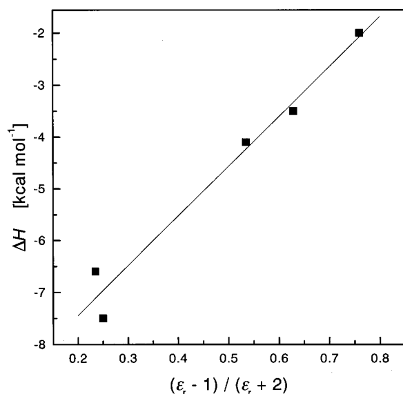
Figure 5. Correlation between \Delta H and (\epsilon_r - 1)/(\epsilon_r + 2) . Data are listed in Table 2 and fitted to a linear relation.
