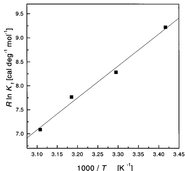
Figure 4. van't Hoff plot for the BPK/TEA complex formation reaction in n -hexane. The \Delta H and \Delta S values were determined from the slope and the intercept, respectively.
