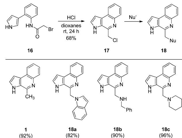
Scheme 3. Synthesis of Marinoquinoline A ( 1 ) and Unnatural Analogs of 6 from a Common Intermediate
