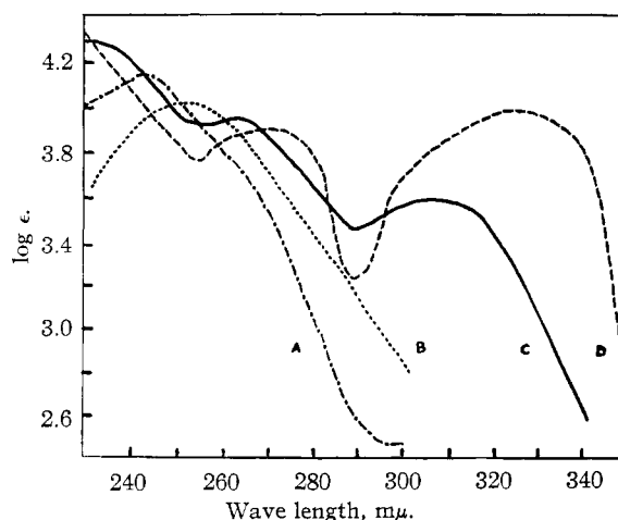
Fig. 1.—Ultraviolet absorption spectra in ethanol: A, \alpha -acetyl- \alpha -methylpropionanilide (IV, \text{R} = \text{R}' = \text{CH}_3 ); B, 3,3,4-trimethyl-1,2,3,4-tetrahydro-2-quinolone (VII); C, 2-hydroxy-3,4-dimethylquinoline (V, \text{R}' = \text{CH}_3 ); D, 3,3-dimethyl-4-methylene-1,2,3,4-tetrahydro-2-quinolone (VIa).
