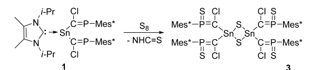
Scheme 2. Synthesis of Dithiadistannetane 3
