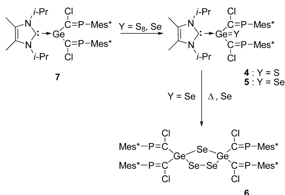
Scheme 3. Synthesis of Chalcogeno (S, Se) Germanium Compounds
