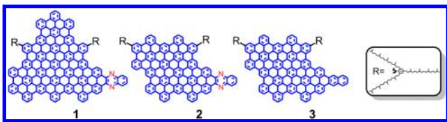
Scheme 1. Structures of N-Doped Graphene QDs 1 , 2 and an Undoped QD 3 for Comparison Studies
