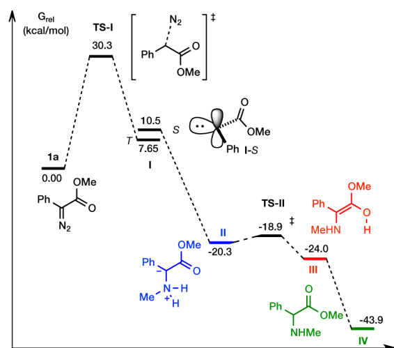
Figure 1. Gas-phase free-energy reaction coordinate diagram for gas-phase reaction between 1a and methylamine at the B3LYP/6-311+G(d,p) level of theory.
