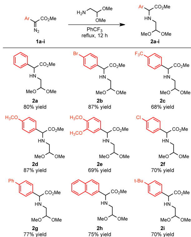
Scheme 1. Thermal N–H Insertions of Aryl Diazoacetates
