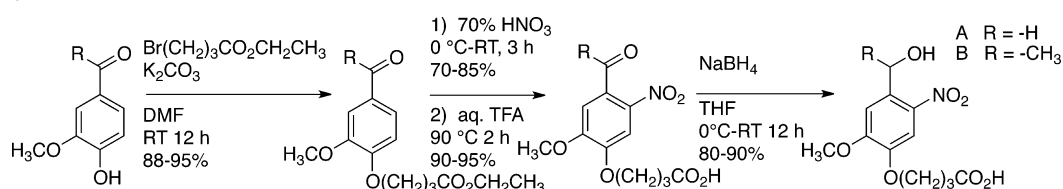
Scheme 1. Synthesis of 4-(4-(Hydroxymethyl)-2-methoxy-5-nitrophenoxy)butanoic acid and 4-(4-(1-Hydroxyethyl)-2-methoxy-5-nitrophenoxy)butanoic acid
