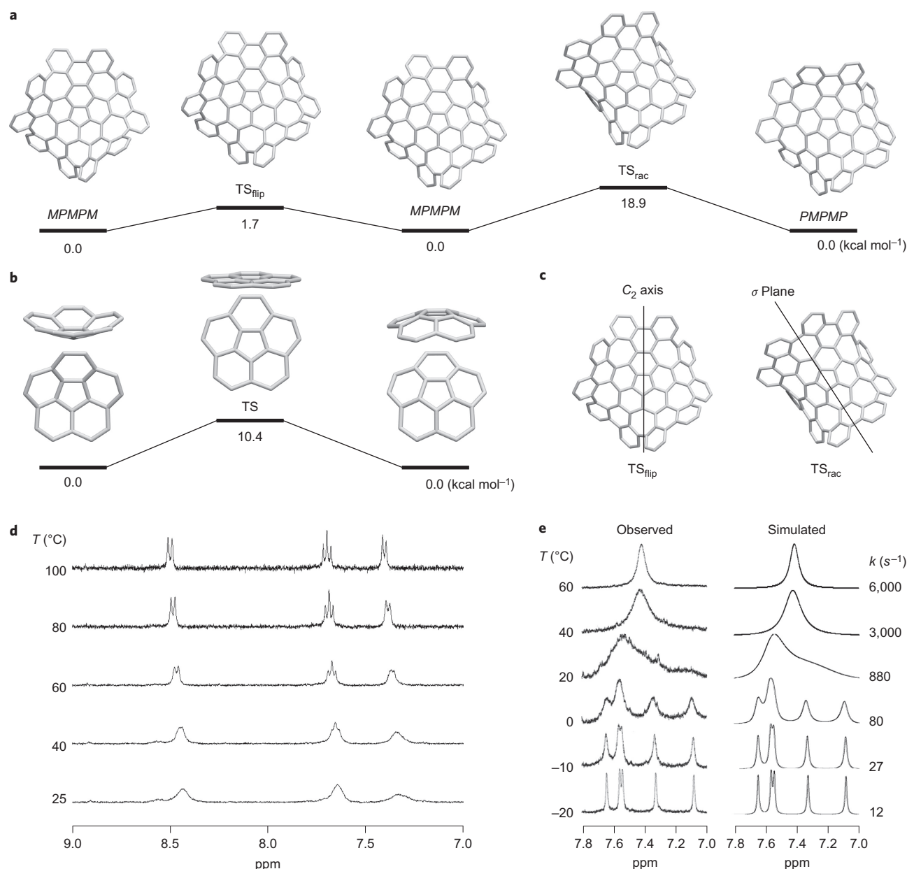
Figure 3 | Conformational flexibility of the grossly warped C 80 H 30 nanographene. a , Bowl-to-bowl inversion (left, MPMPM \rightleftharpoons TS flip \rightleftharpoons MPMPM) and racemization (right, MPMPM \rightleftharpoons TS rac \rightleftharpoons PMPMP) pathways of 4 determined by DFT calculation. Values (kcal mol -1 ) are relative Gibbs free energies ( \Delta G ) at 298.15 K and 1 atm calculated at the B3LYP/6-31G(d) level of theory. The activation energies of bowl-to-bowl inversion and racemization of 4 are predicted to be 1.7 and 18.9 kcal mol -1 , respectively. The bowl-to-bowl inversion barrier of 4 is considerably lower than that of corannulene ( b ). b , Pathway and activation energy (10.4 kcal mol -1 ) of bowl-to-bowl inversion of corannulene determined by DFT calculations at the same level of theory. Both side views and top views of corannulene structures are shown. c , C 2 axis and \sigma plane in the transition states of bowl-to-bowl inversion (TS flip ) and racemization (TS rac ) of 4 , respectively. d , Variable temperature 1 H NMR spectrum of 4 (400 MHz, C 2 D 2 Cl 4 ) reveals the rapid equalization of the ten benzo groups on the perimeter. e , Variable-temperature 1 H NMR spectrum of (t-Bu) 10 C 80 H 20 8 (500 MHz, C 2 D 2 Cl 4 ) gives the experimental values for the activation enthalpy ( \Delta H^\ddagger = 13.6 \pm 1.5 kcal mol -1 ) and entropy ( \Delta S^\ddagger = 0.2 \pm 0.6 cal mol -1 K -1 ) associated with a wave-like motion around the perimeter of the molecule. k , rate constant (s -1 ).
