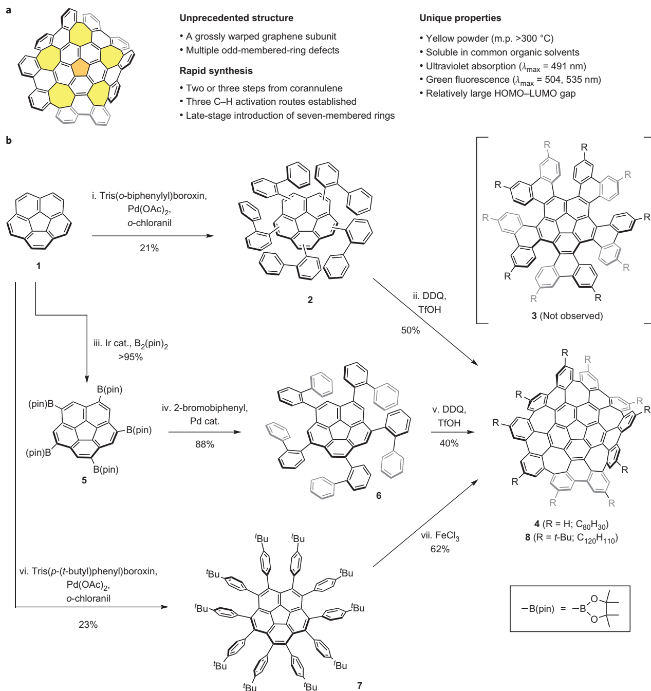
Figure 1 | Structure of 4 , its salient properties and three different synthesis methods. a , Important features of the grossly warped C 80 H 30 nanographene. b , Synthetic routes to C 80 H 30 ( 4 ) and its deca- t -butyl derivative C 120 H 110 ( 8 ) from corannulene ( 1 ). For Route 1, direct fivefold C–H biphenylation, the reaction conditions were (i) tris( o -biphenyl)boroxin (2.0 equiv.), Pd(OAc) 2 (20 mol%), o -chloranil (5.0 equiv.), DCE, 80 °C, 16 h and (ii) DDQ (10 equiv.), trifluoromethanesulfonic acid (TfOH)/CH 2 Cl 2 (5:95), 0 °C, 30 minutes. For Route 2, stepwise fivefold C–H borylation-arylation, the reaction conditions were (iii) (Ir(OMe)(cod)) 2 (20 mol%), B 2 (pin) 2 (5.2 equiv.), 4,4′-dimethylbipyridyl (40 mol%), potassium t -butoxide (10 mol%), tetrahydrofuran (THF), 85 °C, four days, (iv) 2-bromobiphenyl (20 equiv.), Pd 2 (dba) 3 ·CHCl 3 (10 mol%), 2-dicyclohexylphosphino-2′,6′-dimethoxybiphenyl (SPhos, 20 mol%), Cs 2 CO 3 (10 equiv.), toluene/water (2:1), 80 °C, 24 hours and (v) DDQ (10 equiv.), TfOH/CH 2 Cl 2 (5:95), 0 °C, 30 minutes. For Route 3, direct tenfold ‘total’ C–H phenylation, the reaction conditions were (vi) tris( p -( t -butyl)phenyl)boroxin, Pd(OAc) 2 , o -chloranil, DCE, 80 °C, repeat for 3–4 cycles and (vii) FeCl 3 (31 equiv.), CH 2 Cl 2 /nitromethane (115:1), 25 °C, one hour. cod, 1,5-cyclooctadiene; pin, pinacol; dba, dibenzylideneacetone; cat., catalyst; DCE, 1,2-dichloroethane; DDQ, 2,3-dichloro-5,6-dicyanobenzoquinone.
