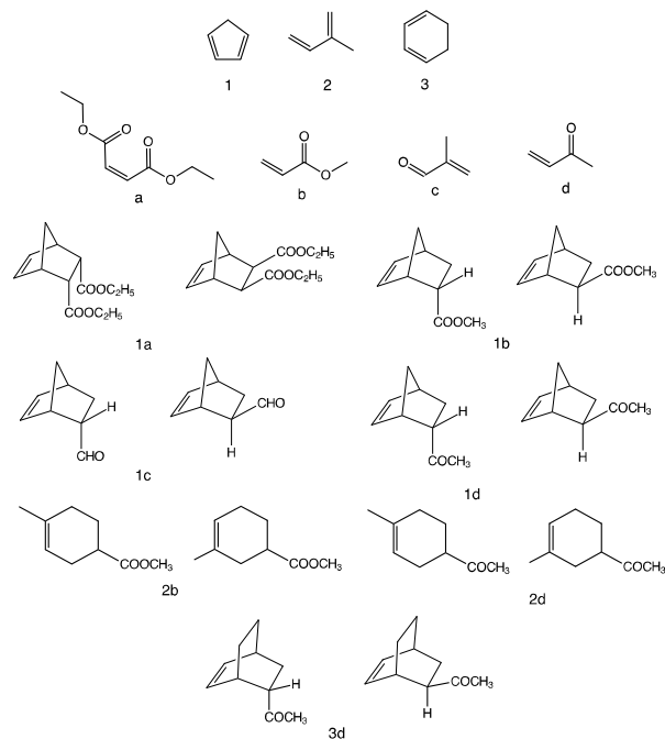
Figure 5 Dienes and dienophiles used in Diels-Alder reaction.
