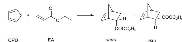
Scheme 2 Diels-Alder cycloaddition of cyclopentadiene to ethyl acrylate.
