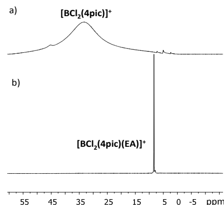
Figure 3 ^{11}\text{B} NMR spectra of a) neat [\text{BCl}_2(4\text{pic})][\text{AlCl}_4] , and b) solution of [\text{BCl}_2(4\text{pic})][\text{AlCl}_4] in ethyl acrylate (EA). Both recorded with external d_6 -DMSO lock.
