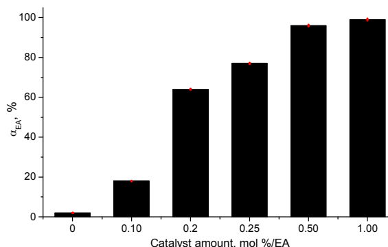
Figure 2. The influence of catalyst loading on the conversion of ethyl acrylate. Reaction conditions: cyclopentadiene (1.586 g, 24 mmol), ethyl acrylate (1.602 g, 16 mmol), catalyst [BCl_2(4pic)][GaCl_4] ; ice bath, 5 min, 1500 rpm, conversion determined by GC.
