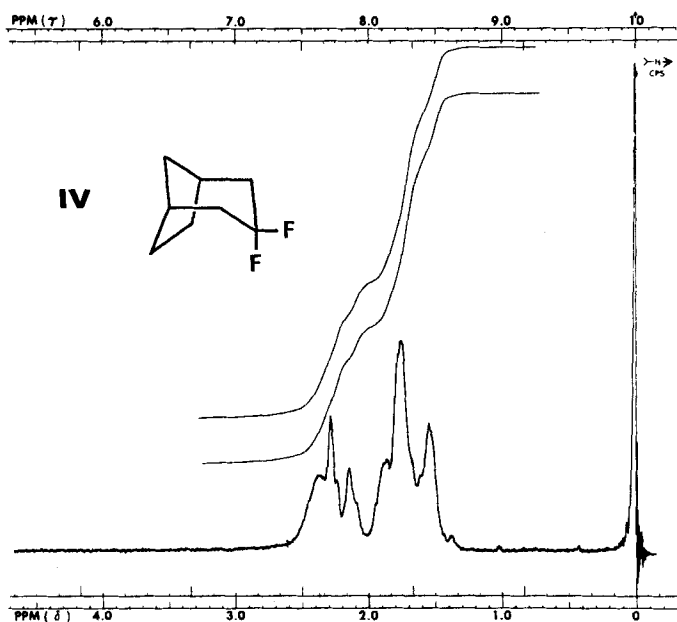
Fig. 2. Proton NMR. spectrum of 3,3-Difluorobicyclo[3.2.1]octane (IV) in \text{CDCl}_3
