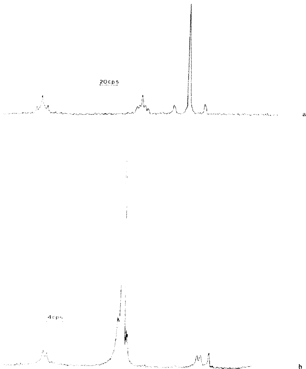
Fig. 1. (a) Proton NMR spectrum of a benzene solution of recrystallized [(\text{CH}_3)_3\text{Sn}]_3\text{SnLi} \cdot (\text{OC}_4\text{H}_9)_3 . For chemical shift data, see Table I and text. (b) Proton NMR spectrum of the methyl group resonance ( \tau = 9.40 ) in a benzene extract of [(\text{CH}_3)_3\text{Sn}]_3\text{SnLi} \cdot (\text{OC}_4\text{H}_9)_3 . The small absorption upfield from the tin-proton coupling doublet is due to an unidentified impurity.
