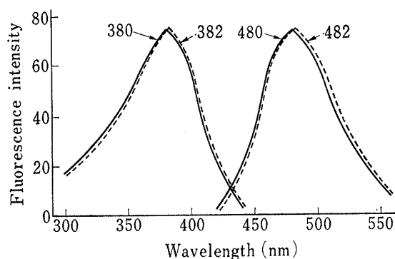
Fig. 1. Excitation and Emission Spectra of BBC and a Reaction Mixture of PIA with HNA
