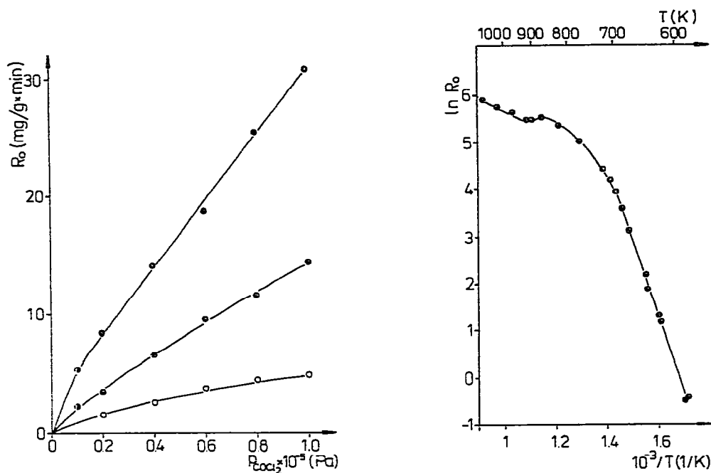
Fig. 2. Specific initial reaction rate vs. partial pressure of phosgene. \circ , 648 K; \ominus , 673 K; \bullet , 698 K.
