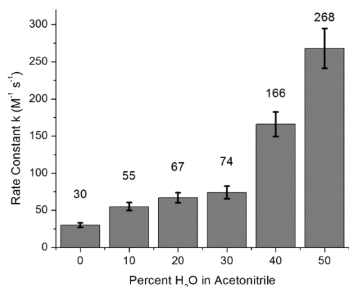
Figure 7. Plot of rate constant k versus water content (v/v) for the reaction between d_0 and d_{60-}\{[\text{CpCo}(\text{P}=\text{O}(\text{OEt})_2)_3]_2\text{Tb}\}^+ \text{Cl}^- ( 5a ) in acetonitrile monitored by ESI MS.
