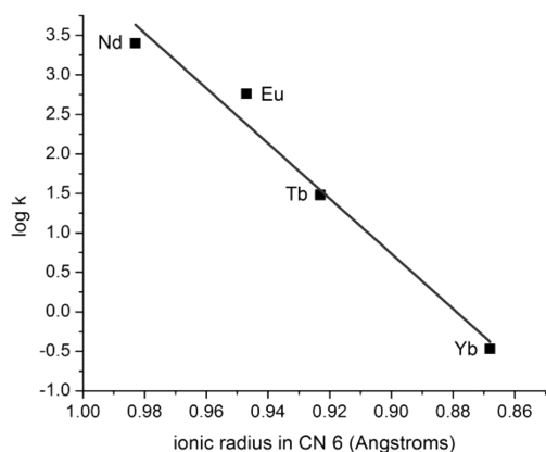
Figure 6. Plot of \log k versus ionic radius (Å) for the reaction between d_0 and d_{60-}\{[\text{CpCo}(\text{P}=\text{O}(\text{OEt})_2)_3]_2\text{Ln}\}^+ \text{Cl}^- ( 3a–6a ) in acetonitrile monitored by ESI MS.
