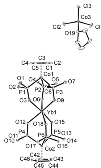
Figure 1. ORTEP3 14 plot of \{[\text{CpCo}(\text{P}=\text{O}(\text{OPh})_2)_3]_2\text{Yb}\}^+ \{\text{CoCl}_3(\text{THF})\}^- \cdot 2\text{C}_6\text{H}_6 , 7 (50% probability ellipsoids; phosphite phenyl groups and benzenes of solvation omitted for clarity).
