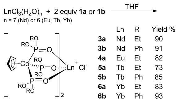
Scheme 2. Synthesis of Lanthanide Complexes, \{[\text{CpCo}(\text{P}=\text{O}(\text{OR})_2)_3]_2\text{Ln}\}^+ \text{Cl}^-
