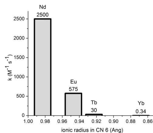
Figure 5. Plot of rate constant k versus ionic radius (Å) for the reaction between d_0 and d_{60}\text{-}\{[\text{CpCo}(\text{P}=\text{O}(\text{OEt})_2)_3]_2\text{Ln}\}^+ \text{Cl}^- ( 3a – 6a ) in acetonitrile monitored by ESI MS.
