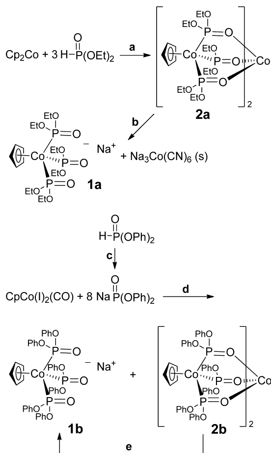
Scheme 1. Synthesis of Ligands, [\text{CpCo}(\text{P}=\text{O}(\text{OR})_2)_3]^- \text{Na}^+ , 1a ( \text{R} = \text{Et} ) and 1b ( \text{R} = \text{Ph} ) a
