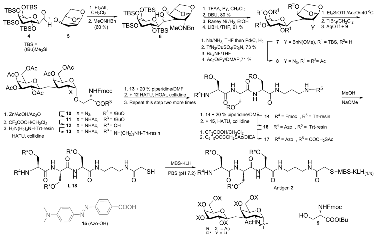
Scheme 1. Synthesis of triglycopeptide 18 and the preparation of the corresponding antigen 2 : Triphenylmethyl (Trt); 2-(1 H -7-azabenzotriazol-1-yl)-1,1,3,3-tetramethyl uronium hexafluorophosphate methanaminium (HAUT); trifluoroacetic anhydride (TFAA); 1,8-diazabicyclo[5.4.0]undec-7-ene (DBU); 4-dimethylaminopyridine (DMAP); N,N -diisopropylethylamine, or Hünig's base (DIEA); phosphate buffered saline (PBS).
