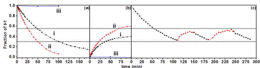
Figure 3. Plots of the fraction of t -1 against the irradiation time for (a) t -1 → c -1 at 340 nm, (b) c -1 → t -1 at 250 nm, and (c) t -1 → c -1 // c -1/H + → t -1/H + // t -1 → c -1 // c -1/H + → t -1/H + // t -1 → c -1 at alternating 340 and 250 nm in acetonitrile. The substrate concentration is 1.0 \times 10^{-5} M. The black (i) and red (ii) curves are at 0.0 and 10.0 equiv of HCl, respectively, and the blue (iii) curves are at 10.0 equiv of HCl in the dark.
