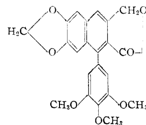
VI, dehydroanhydricropodophyllin
