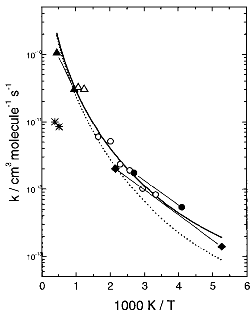
Figure 3. Comparison of k_1 value for the H + H 2 S reaction. (○) this work; (◆) ref 19; (●) ref 20; (▲) ref 3; (*) ref 28; (Δ) ref 27; (dotted line) TST calculation with E_0^+ = 16.0 kJ/mol; (solid line) TST calculation with E_0^+ = 14.4 kJ/mol.
