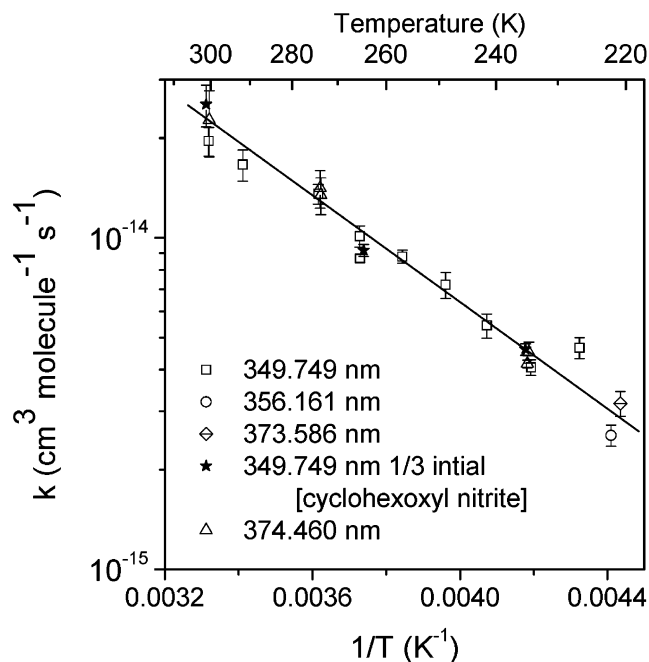
Figure 4. Arrhenius plot showing the temperature dependence of the rate constant for the reaction of cyclohexoxy with \text{O}_2 .
