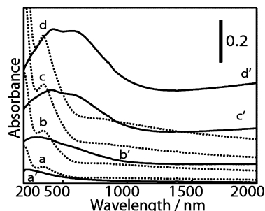
Figure 4. UV-vis-IR absorption spectra for layer-by-layer nanosheet films having layer numbers of (a and a') 1, (b and b') 3, (c and c') 6, and (d and d') 10 before (broken line) and after (solid line) reduction.
