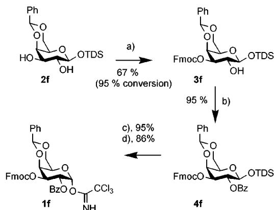
Scheme 3 a
