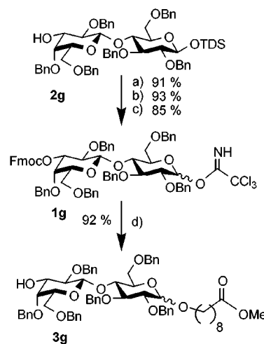
Scheme 4. Glycosylation in Solution a
