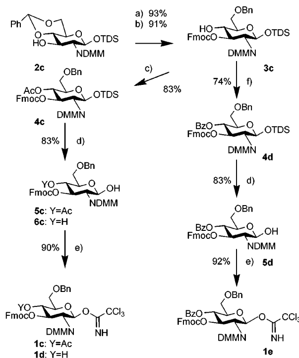
Scheme 2 a
