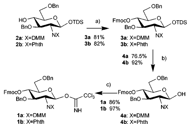
Scheme 1 a
