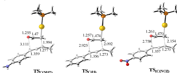
Figure 5. B3LYP/LANL2DZ TSs for the gold(I)-catalyzed Claisen-rearrangements emanating from a Au(I)-VE complex.
