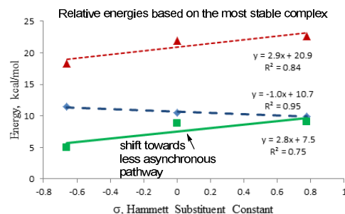
Figure 7. Correlation of Hammett substituent constants and the activation barrier for the three mechanisms (activation energies adjusted based on Curtin-Hammett correction). Red dashed line correspond to Au(I)-VE mechanism, blue-dashed line correspond to cyclization-mediated rearrangement and the solid green line represents cation-accelerated oxonia Claisen rearrangement.
