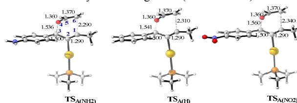
Figure 1. B3LYP/LANL2DZ TSs for the gold(I)-catalyzed cyclization-mediated Claisen-rearrangements of the three aryl-substituted propargyl vinyl ethers.
