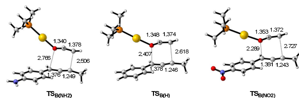
Figure 3. B3LYP/LANL2DZ TSs for the Au(I)-catalyzed cation accelerated oxonia Claisen-rearrangements
