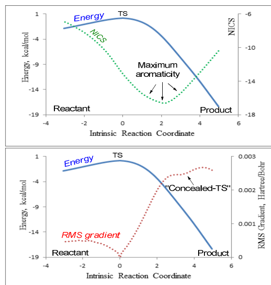
Figure 2. B3LYP/LANL2DZ IRC results for the gold(I)-coordinated substrate 15 (path A).
