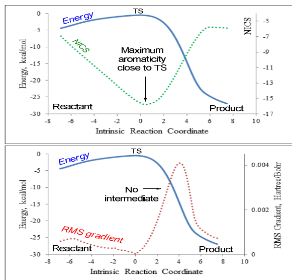
Figure 4. B3LYP/LANL2DZ IRC calculations for the gold(I)-coordinated substrate 15 (path B).
