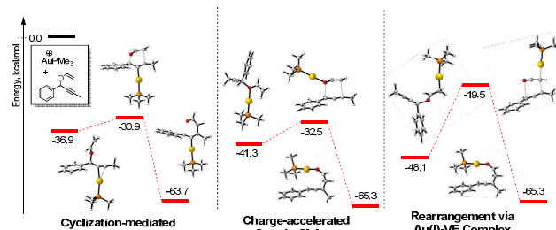
Figure 6. Curtin-Hammett analysis of the three mechanisms. Energies for the three pathway are given relative to the two non-interacting reagents.
