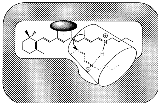
Figure 1. Latchet model for regioselective photoisomerization.
