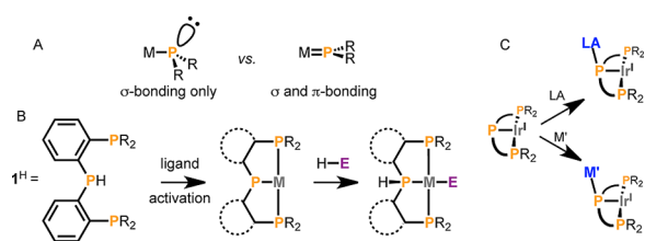
Figure 1. (A) Trigonal pyramidal vs trigonal planar terminal phosphide coordination, (B) concept of a cooperative \text{P}^{\text{H}}/\text{P}^- couple based on 1^{\text{H}} , and (C) metalloligand reactivity of a terminal \text{Ir}^{\text{I}}(\text{PR}_2) species.
