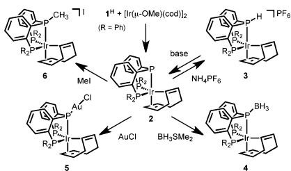
Scheme 1. Synthesis and Versatile Reactivity of Complex 2
