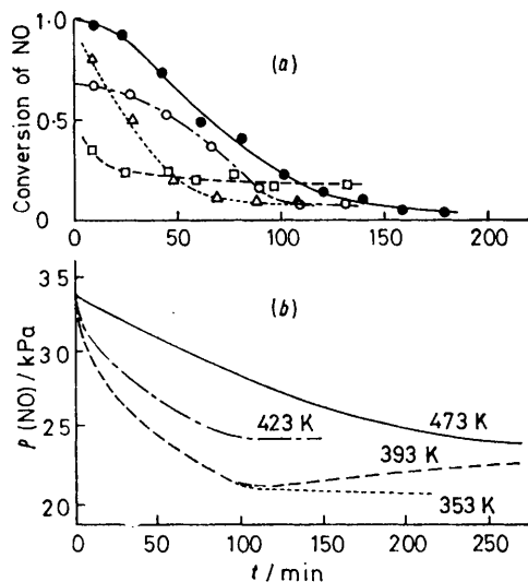
FIGURE 1 Reaction of \text{Ag}_2\text{O} with NO at 353 ( \Delta ), 393 ( \square ), 423 ( \circ ), and 473 K ( \bullet ) in the flow (a) and static systems (b)
