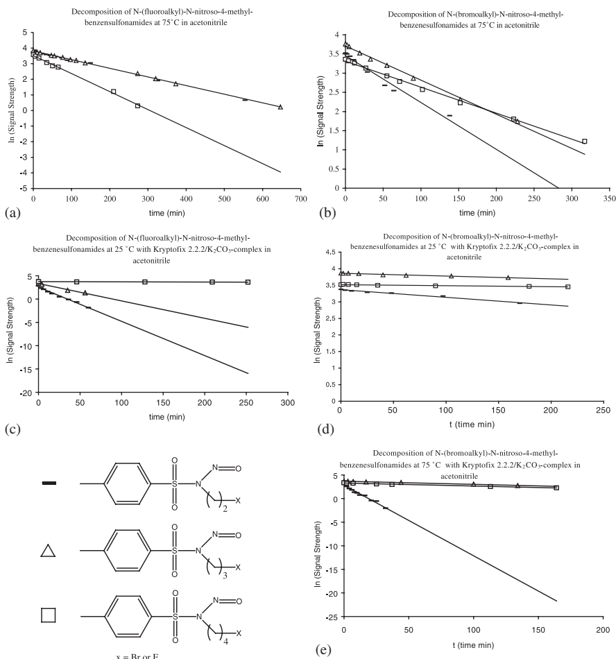
Figure 1. Decomposition studies of N -(halogenoalkyl)- N -nitroso-4-methyl benzenesulfonamides (fluoro-derivatives 11–13 and bromo-derivatives 14–16 ): (a) 11–13 , acetonitrile, 75 °C (b) 14–16 , acetonitrile, 75 °C, (c) 11–13 , acetonitrile, 25 °C, Kryptofix ® 2.2.2./ \text{K}_2\text{CO}_3 (d) 14–16 , acetonitrile, 25 °C, Kryptofix ® 2.2.2./ \text{K}_2\text{CO}_3 (e) 14–16 , acetonitrile, 75 °C, Kryptofix ® 2.2.2./ \text{K}_2\text{CO}_3
