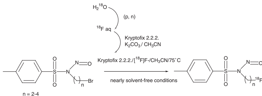
Scheme 3. Radioactive labelling of bromo precursors 14–16 applying nearly solvent-free conditions to obtain N -([ ^{18}\text{F} ]fluoroalkyl)- N -nitroso-4-methyl-benzenesulfonamides ( 11–13 )
