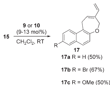
Scheme 4. RCEM of 15 .
