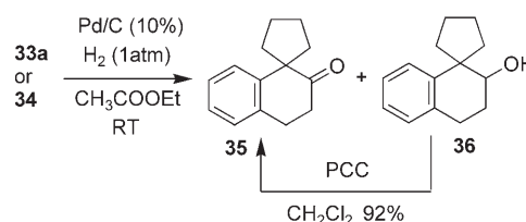
Scheme 8. Pd/C-catalyzed hydrogenations of 33a and 34 .
