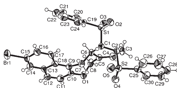
Figure 2. ORTEP diagram of compound 26 .
