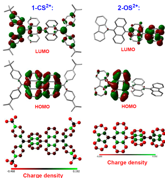
Figure 11. Calculated frontier molecular orbital profiles and the Mulliken charge density distribution of 1\text{-CS}^{2+} and 2\text{-OS}^{2+} .
