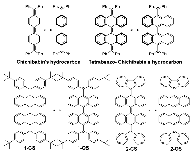
Chart 1. Resonance Structures of Chichibabin's Hydrocarbon, Tetrabenzo-Chichibabin's Hydrocarbons, and Its Derivatives 1-CS/1-OS and 2-CS/2-OS
