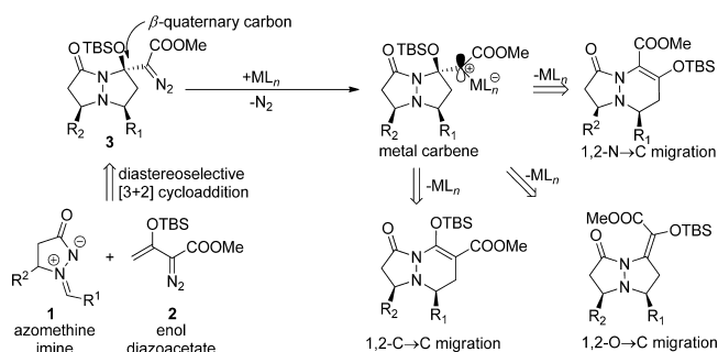
Scheme 1. Strategy for the Synthesis of \alpha -Diazooacetates Bearing \beta -Quaternary Carbons and Chemoselectivity of Competitive 1,2-C→C, -O→C, and -N→C Migrations
