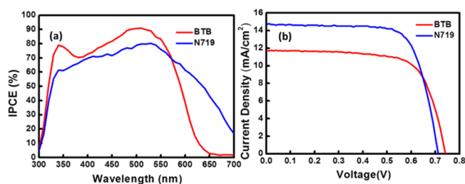
Figure 4. (a) IPCE spectra of DSSCs based on BTB (red) and N719 (blue). (b) Current–voltage curves for DSSCs incorporating BTB (red) and N719 (blue) under AM 1.5 G simulated sunlight.
