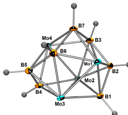
Figure 3. Molecular structure of [(\text{Cp}^*\text{Mo})_4\text{B}_4\text{H}_4(\mu_4\text{-BH})_3] , 5 . \text{Cp}^* are omitted for clarity. Selected bond lengths (Å) and angles (deg): Mo(1)–Mo(3) 2.659 (10), Mo(2)–Mo(4) 2.651 (9), Mo(2)–Mo(3) 2.847(10), Mo(1)–B(1) 2.220(9), Mo(1)–B(2) 2.136(11), Mo(1)–B(3) 2.309(10), Mo(2)–B(2) 2.158(9), Mo(3)–B(6)–Mo(1) 69.71(11).
