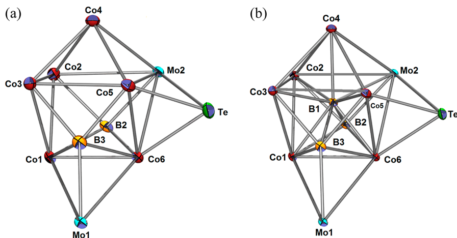
Figure 7. Molecular structure of [(\text{Cp}^*\text{MoCO})_2\text{B}_3\text{H}_2(\mu_3\text{-Te})(\mu\text{-CO})_4\{\text{Co}_6(\text{CO})_8\}] , 8 . \text{Cp}^* and CO are omitted for clarity. (a) Without interstitial boron atom and (b) with encapsulated boron atom. Selected bond lengths (Å) and angles (deg): Co1–Co2 2.647(7), Co3–Co5 2.791(6), Mo2–B2 2.280(4), Co5–Co6 2.562(7), Co6–B2 2.109(4), Mo1–Co6 2.731(5), Co5–Te 2.453(5), B1–B2 1.750(5), B1–Co1 2.140(4); Co6–Mo1–Co1 55.604(13).
