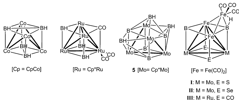
Scheme 1. Synthesis of Compounds 2–5
