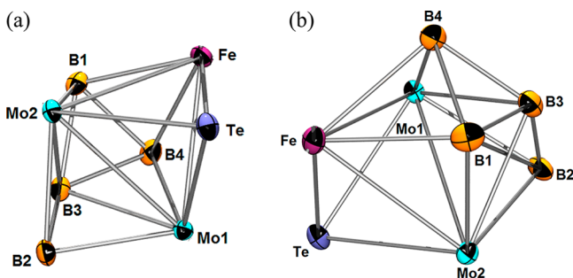
Figure 4. Molecular structure of [(\text{Cp}^*\text{Mo})_2(\text{BH})_4(\mu_3\text{-Te})\{\text{Fe}(\text{CO})_3\}] , 6. \text{Cp}^* are not shown for clarity. (a) Cubane view; (b) biccapped octahedron view. Selected bond lengths (Å) and angles (deg): Mo(1)–Mo(2) 2.9518(11), Mo(2)–Te(1) 2.6641(10), Fe(1)–Mo(1) 2.7985(16), Fe(1)–Te(1) 2.6270(15), Mo(1)–B(3) 2.323(11), Fe(1)–B(1) 2.226(13), B(1)–B(2) 1.749(16), B(1)–B(3) 1.741(16); Fe(1)–Te(1)–Mo(2) 64.25(4).
