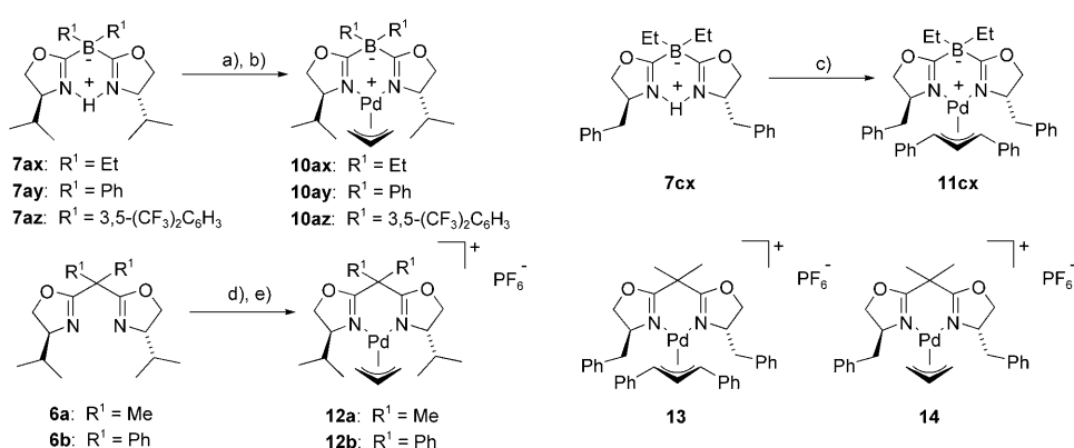
Scheme 2. Synthesis of box and borabox palladium complexes. a) n BuLi, THF, 0°C; b) [Pd(C_3H_5)Cl]_2 , THF, RT; c) K_2CO_3 , [Pd(C_3H_5)Cl]_2 , CH_2Cl_2 /THF/methanol, 50°C; d) [Pd(C_3H_5)Cl]_2 , CH_2Cl_2 , RT; e) AgPF_6 , THF, RT. Complexes 13 , 14 : ref. [7].
