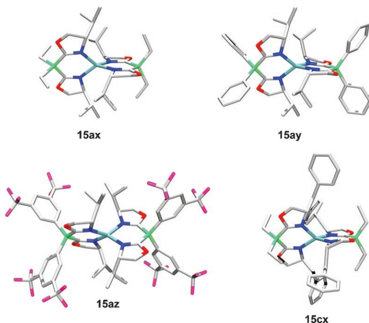
Figure 5. Crystal structures of four different homoleptic borabox copper complexes. \text{CF}_3 groups in 15az were disordered.
