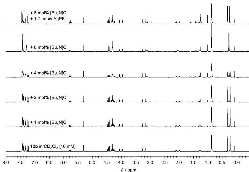
Figure 1. ^1H NMR spectra (500 MHz, CD_2Cl_2 , 295 K) showing a titration experiment of complex 12b (16 mM) with a solution of [Bu_4N]Cl (10 mM in CD_2Cl_2 ). Spectrum at top: addition of [Bu_4N]Cl (8 mol %) and AgPF_6 (1.7 equiv).
