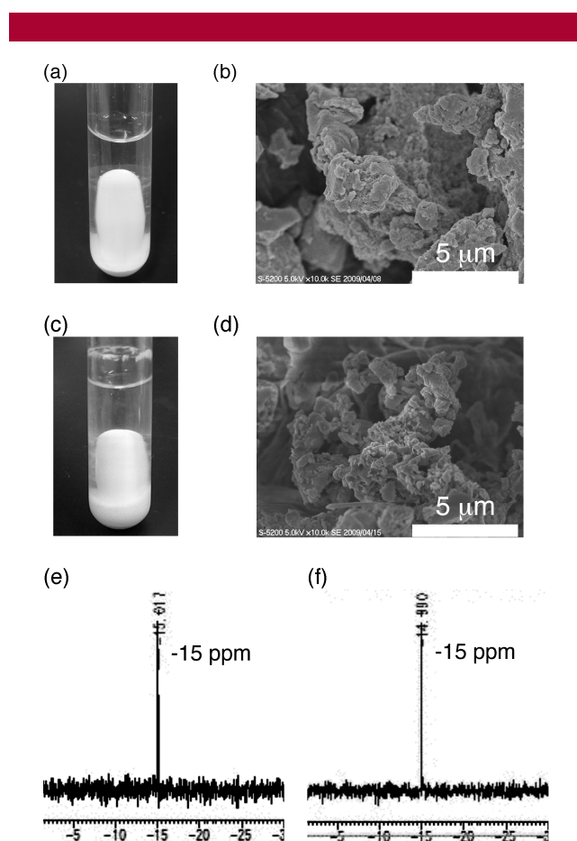
Figure 1. Photo, SEM images, and 31 P{ 1 H} NMR charts of the catalyst 3 (before and after catalytic use): (a) a photo image before use; (b) a SEM image before use; (c) a photo image after use; (d) a SEM image after use; (e) 31 P{ 1 H} NMR before use; and (f) 31 P{ 1 H} NMR after use.
