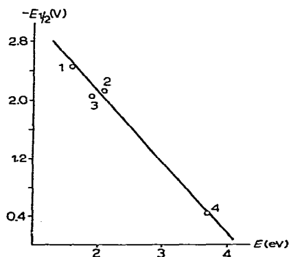
Fig. 2. A plot of the E_{1/2} value of R_2Hg (in DMF, 0.1 N Et_4NClO_4 ) versus the electron affinity of the R\cdot radical. 1, R=C_6H_5\cdot ; 2, R=C_3H_5\cdot ; 3, R=C_6H_5CH_2\cdot ; 4, R=CN\cdot .
