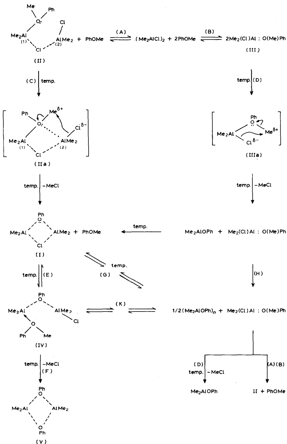
SCHEME 1. Proposed scheme for the cleavage of anisole by dimethylaluminium chloride.
