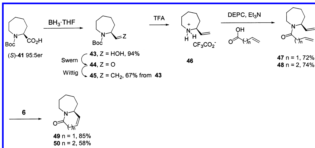
Scheme 6
