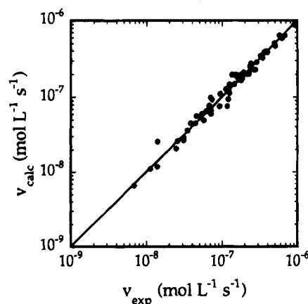
Figure 3. Plot of v_{\text{calc}} , the initial rate calculated using eq 3 and the best fit values for k_3 and k_4 , vs v_{\text{exp}} , the experimental initial rate. The values of k_1 = 42.2 L mol -1 s -1 , k_{-1} = 2.62 s -1 , k_2 = 5.2 L mol -1 s -1 , and k_{-2} = 0.039 s -1 in eq 3 were fixed. The best fit values for k_3 and k_4 were, 0.0562 \pm 0.0031 L mol -1 s -1 and 0.1305 \pm 0.0049 L mol -1 s -1 , respectively. This global fitting included data from 78 experiments. The plot is shown on a log–log scale to allow the full range of variations to be seen.
