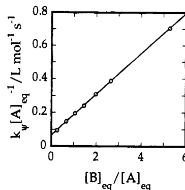
Figure 2. Plot of k_{\psi}/[\text{A}]_{\text{eq}} vs [\text{B}]_{\text{eq}}/[\text{A}]_{\text{eq}} for the oxidation of \text{Cl}^- with [\text{MTO}] = 0.10 \text{ mM} , [\text{Cl}^-] = 0.024\text{--}0.100 \text{ M} , and [\text{H}_2\text{O}_2] = 0.002\text{--}0.040 \text{ M} . The least-squares fit has intercept k_3 = 0.0646 \pm 0.0015 \text{ L mol}^{-1} \text{ s}^{-1} and slope k_4 = 0.1214 \pm 0.0006 \text{ L mol}^{-1} \text{ s}^{-1} .
