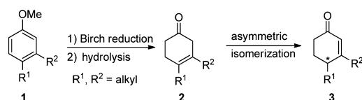
Scheme 1. Asymmetric Synthesis of Cyclohex-2-enones from Anisoles 1
