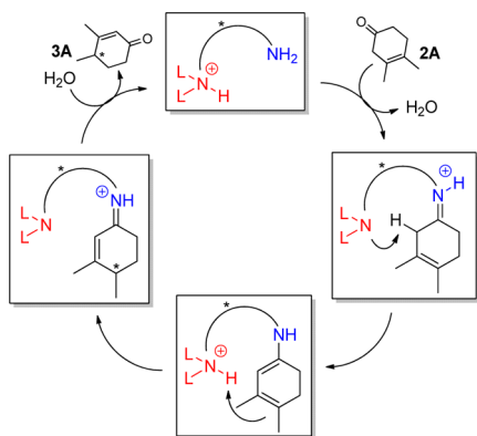
Scheme 2. Proposed Mechanism for Isomerization of 2A via an Enamine Pathway by a Chiral Primary–Tertiary Diamine
