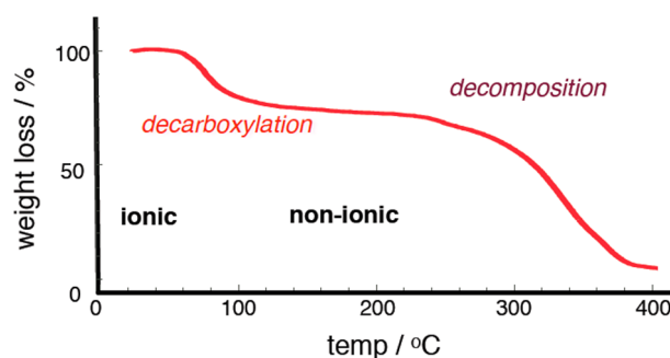
Figure 1. TGA profile of 4 under nitrogen atmosphere (heating rate of 10 °C·min −1 ).
