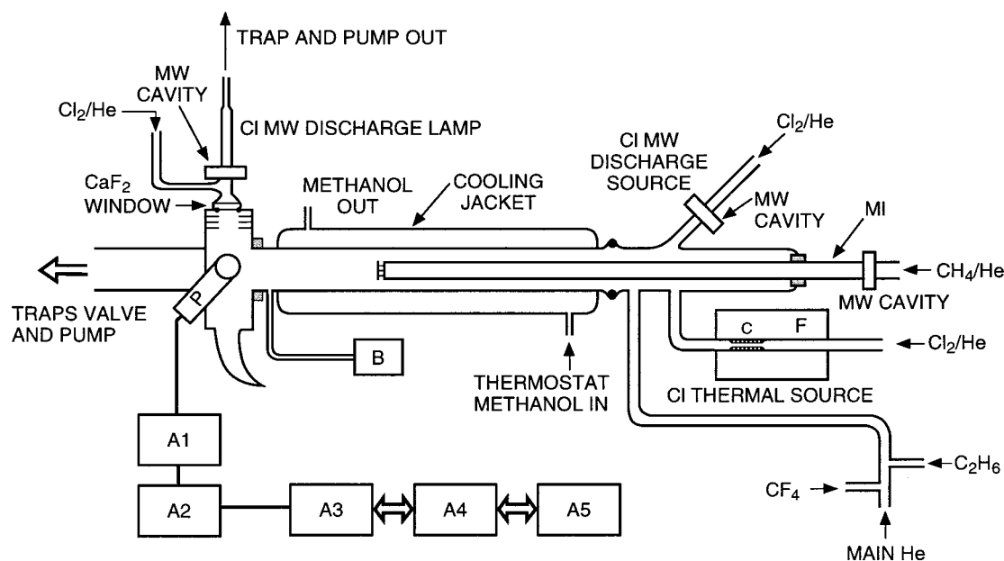
Figure 1. Schematic diagram of discharge flow resonance fluorescence apparatus: B—Baratron pressure gauge ( 1\sim 10 Torr); MI—movable injector for addition of \text{CH}_4 + \text{He} during \text{Cl} + \text{CH}_4 kinetics runs, \text{F}_2 + \text{He} during \text{Cl} atom calibration runs, and \text{Cl}_2 + \text{He} during \text{Cl} atom wall loss runs; F—furnace; C—capillary tube; P—photomultiplier with \text{BaF}_2 filter; A1—fast-preamplifier; A2—amplifier/discriminator; A3—dual counter/timer; A4—interface; A5—computer.
