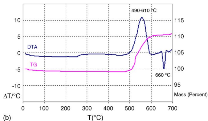
Fig. 1. TG and DTA curves for pure aluminum powder: (a) 5 \mu\text{m} particle size and (b) 18 \mu\text{m} particle size (sample mass, 4.0 mg; heating rate, 10^\circ\text{C}/\text{min} ; air atmosphere).
