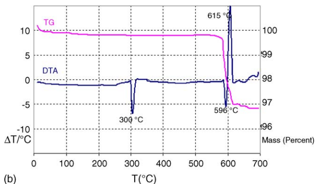
Fig. 3. TG and DTA curves for mixture of aluminum powder with 5 \mu\text{m} particle size and potassium perchlorate with mass ratio (a) 30:70 and (b) 50:50 (sample mass, 4.0 mg; heating rate, 10^\circ\text{C}/\text{min} ; air atmosphere and potassium perchlorate with 50 \mu\text{m} particle size).
