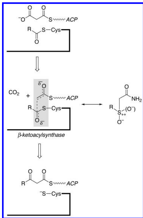
Scheme 1
