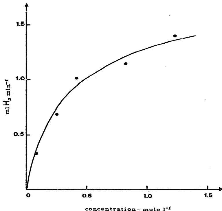
Fig. 1. Plot of the rate of hydrogenation of cyclohexene (ml H 2 absorbed/min) vs olefin concentration, in benzene at 25^\circ\text{C} with 0.2 g R_1 .
