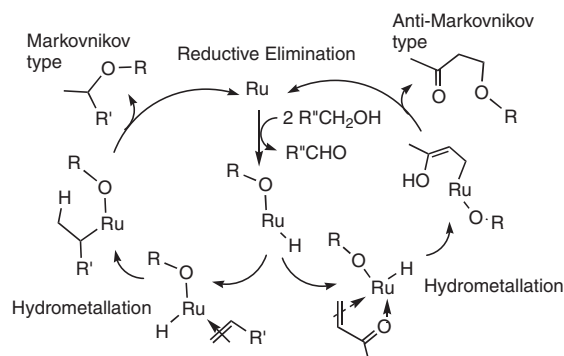
Scheme 4. Proposed catalytic cycle for alkoxylation.
