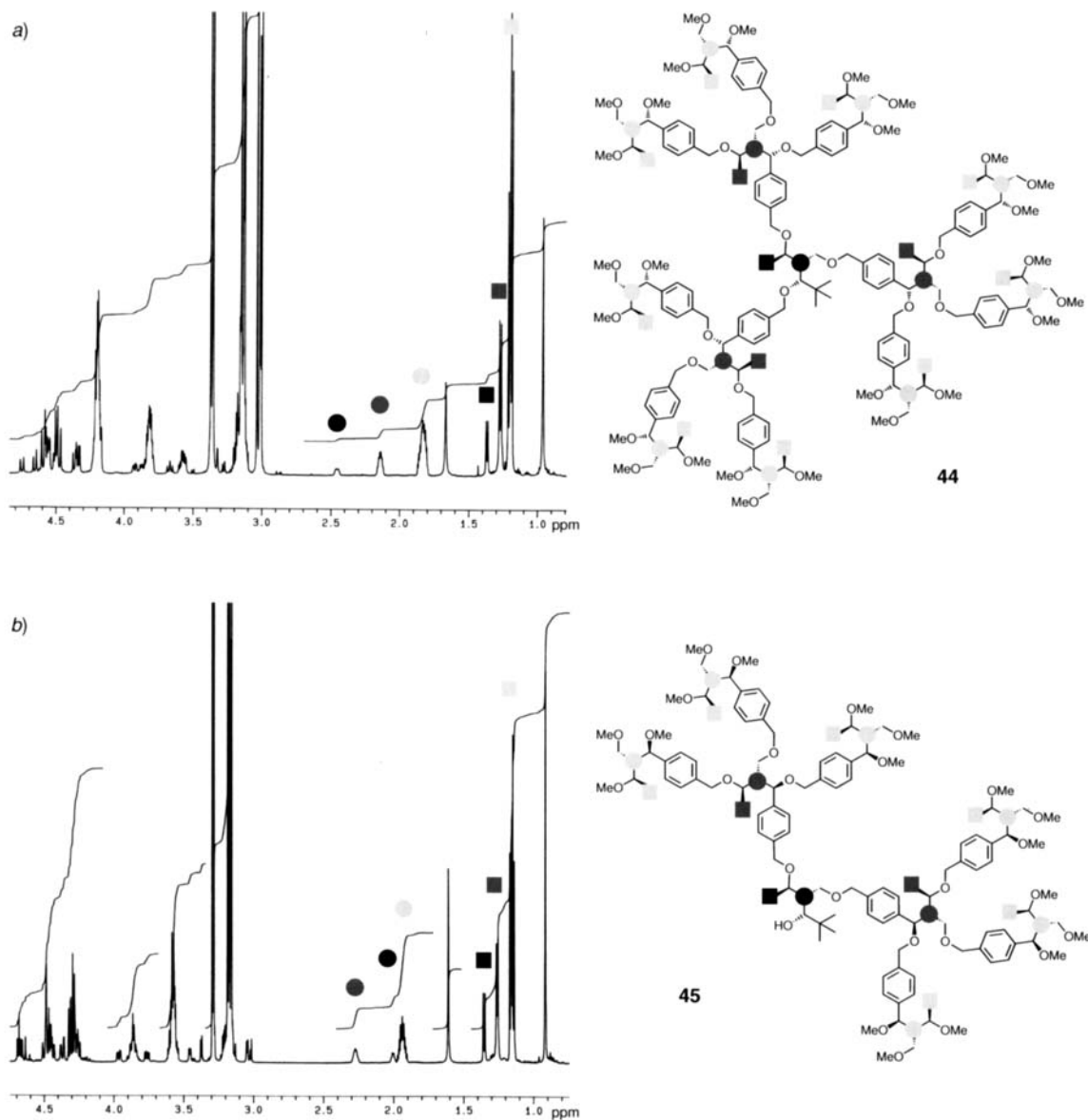
Fig. 2. Part of the 500-MHz ^1\text{H} -NMR spectra of the 2nd-generation dendrimer 44 (a) and the dendritic compound 45 (b) measured in \text{CDCl}_3 . The labelling of signals or groups of signals refers to the sets of Me groups (masked as squares) and of CH groups (masked as circles) in the corresponding formulae (see text).
