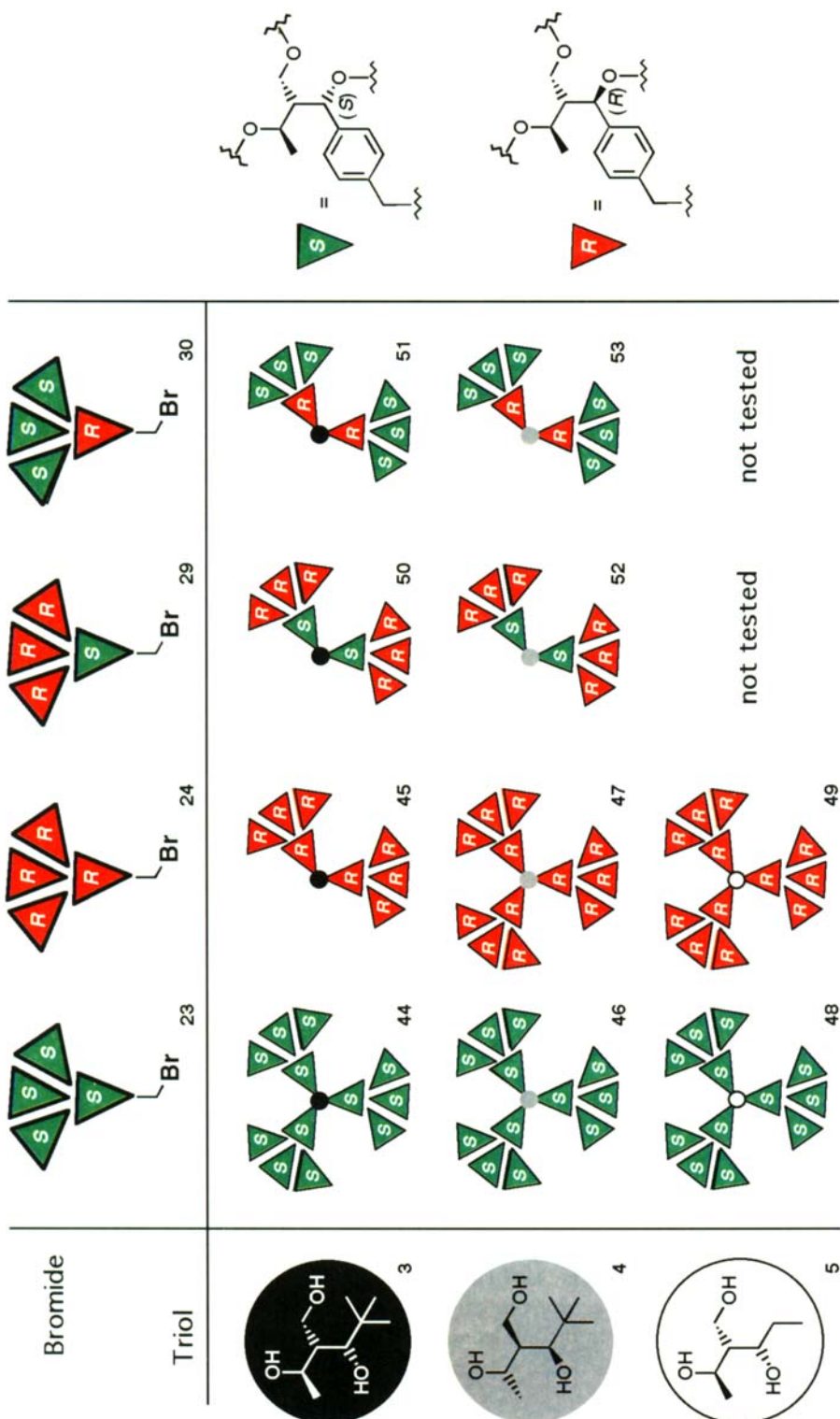
Scheme 5. Combination of Diastereoisomeric 2nd-Generation Benzylc Bromides (23, 24, 29, and 30) with Different Triols (3, 4 (ent-3), 5) leading to 'Doubly Coupled' Dendritic Derivatives (45, and 50–53) in 53–88% Yield and to 'Fully Coupled' Dendrimers (44, and 46–49) in 46–56% Yield. All reactions were carried out under the same coupling reactions, i.e., 9 equiv. NaH, 3.5 equiv. bromide, THF, reflux.
