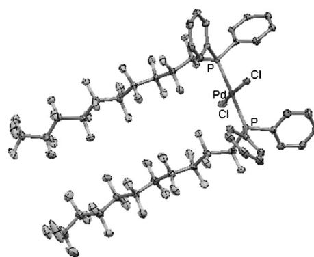
Figure 3. ORTEP representation (thermal ellipsoids at 50% probability) of 7a . R = 0.0346, R w = 0.1059, GOF = 1.132.
