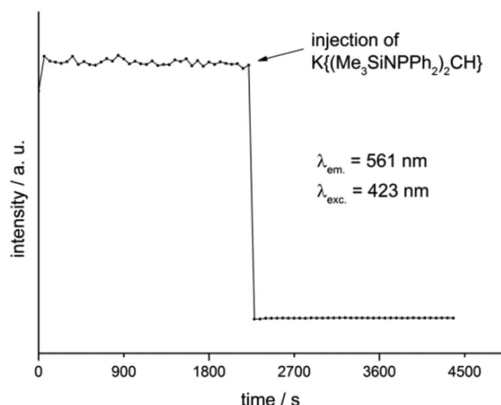
Figure 6. Treatment of 1a with \text{K}\{(\text{Me}_3\text{SiNPPH}_2)_2\text{CH}\} to form 3a resulted in an immediate quenching of the luminescence.
