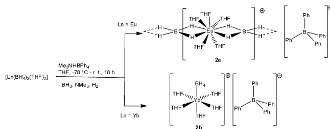
Scheme 2. Syntheses of 2a,b
