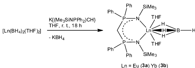
Scheme 3. Synthesis of 3a,b
