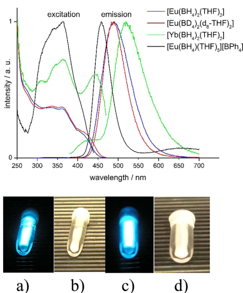
Figure 2. (Top) Excitation/emission spectra of complex hydrides. (Bottom) Photographs of 1a (a,b) and 1a' (c,d) under 366 nm excitation (a,c) and daylight (b,d).
