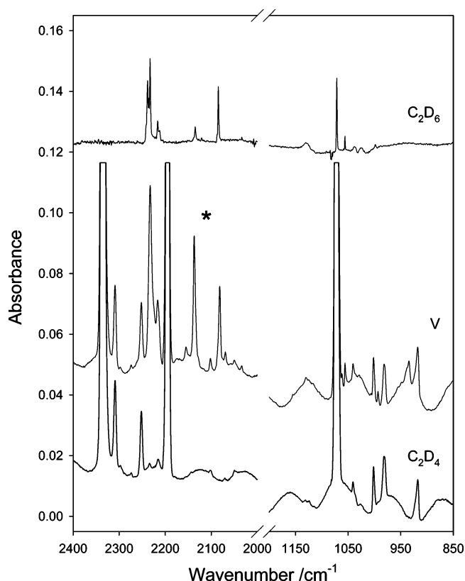
Figure 4. Portions of the FTIR absorption spectra of argon matrices containing (from bottom to top) 10% perdeuterioethene, 10% perdeuterioethene with V atoms, and 0.1% perdeuterioethane. The asterisk denotes a feature due to matrix-isolated CO, generated by thermal desorption of CO in the apparatus during sample preparation.
